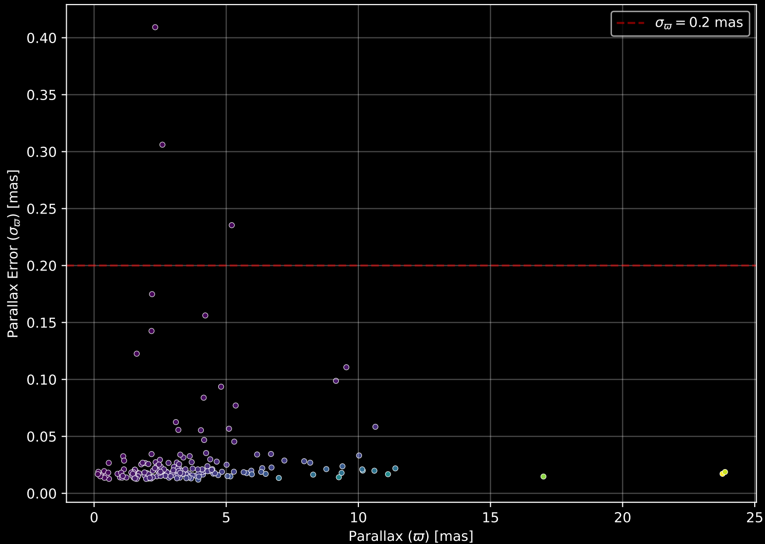
APOGEE DR17 Field: [179+57_MGA] Parallax Quality (n= 188)
