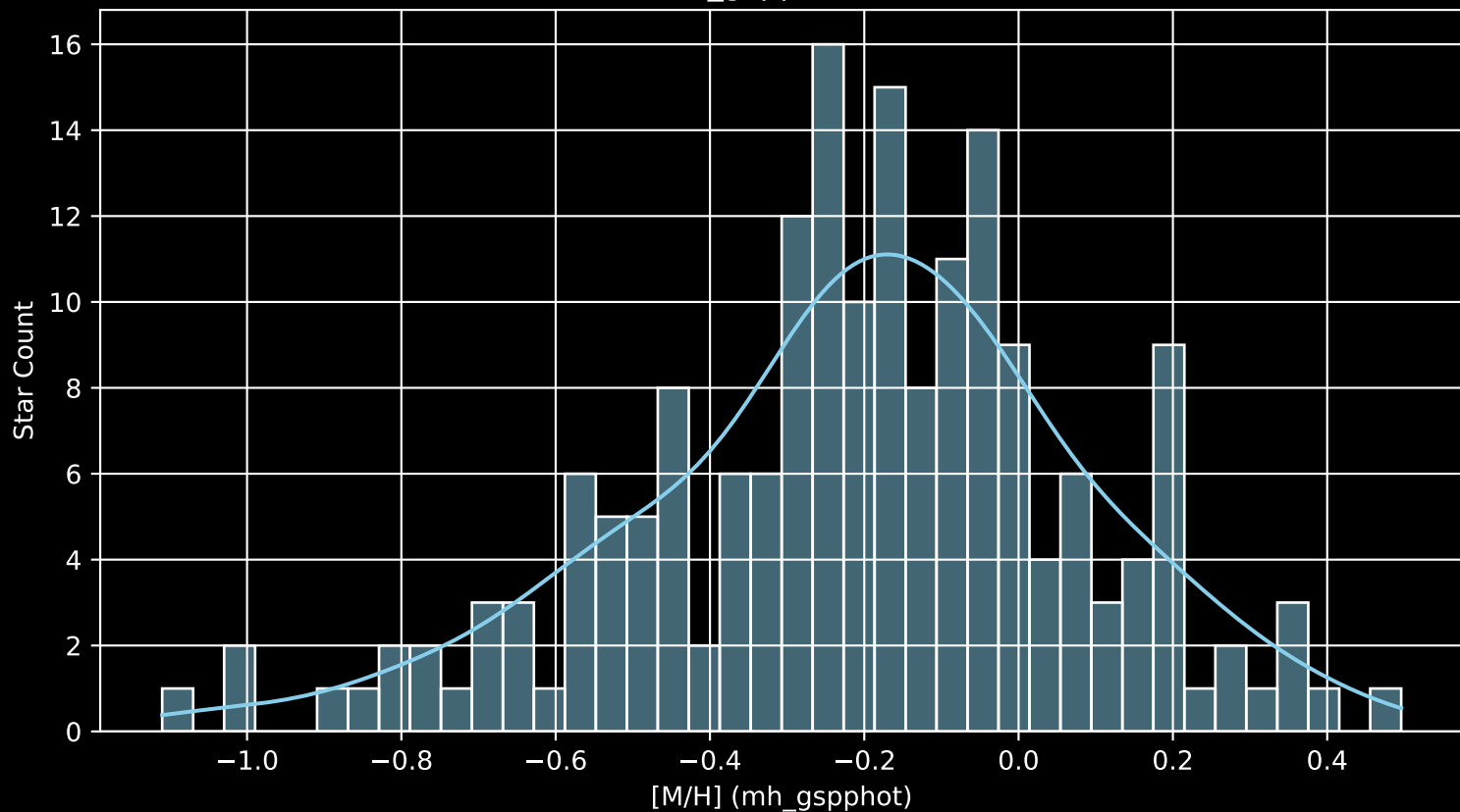
APOGEE DR17 Field: [179+57_MGA [M/H] (mh_gspphot) (n= 185)
