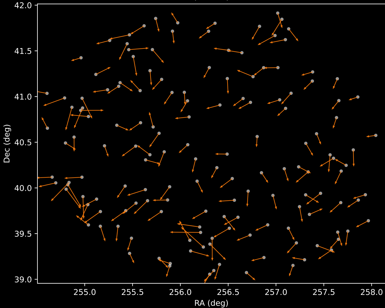
APOGEE DR17 Cluster 2 Proper Motion Vectors (n=151)
