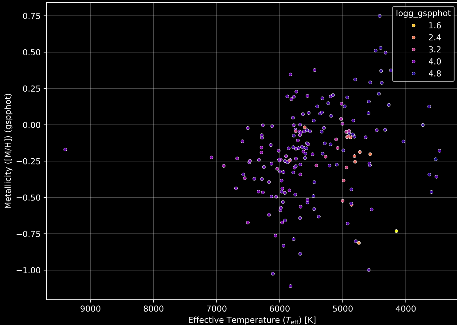
APOGEE DR17 Field: [179+57_MGA] Stellar Population Parameters (n= 188)
