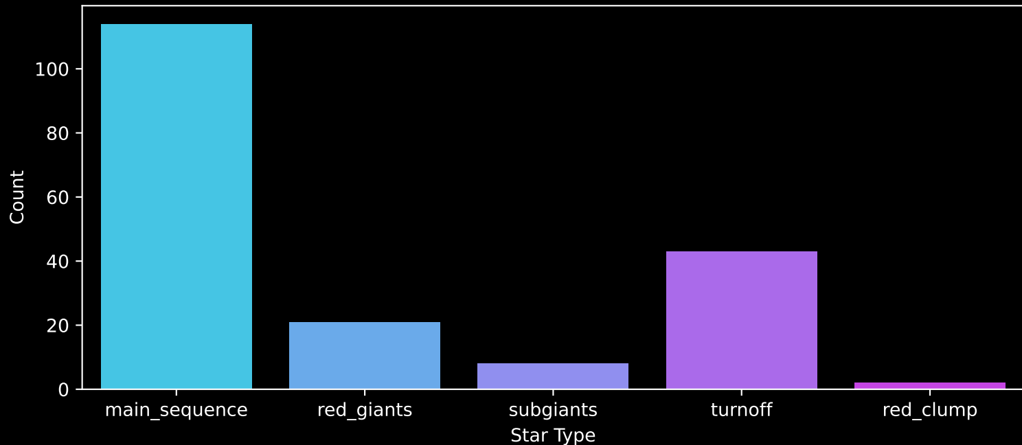
APOGEE DR17 Field: [179+57_MGA] Count plot of Star Type
