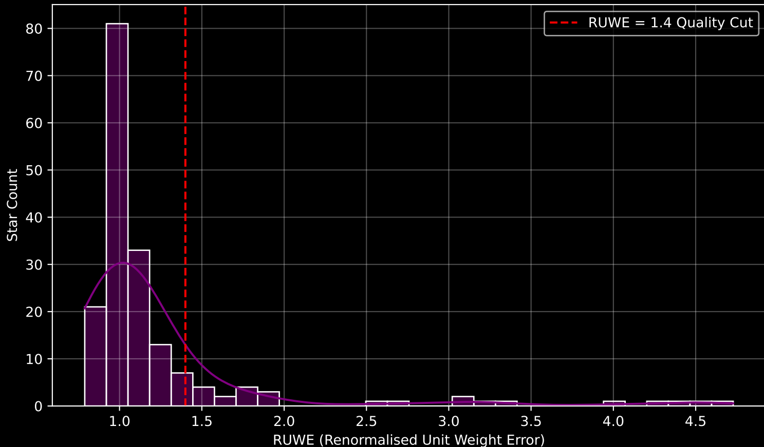
GAPOGEE DR17 Field [179+57_MGA] RUWE Distribution (n= 179)
