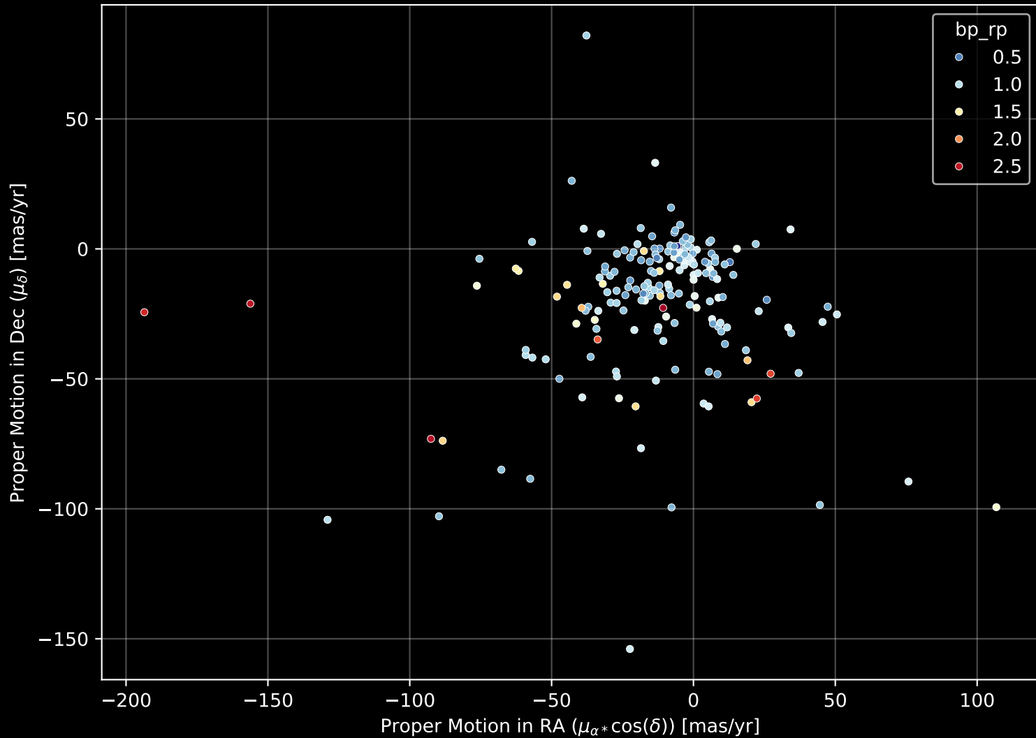
APOGEE DR17 Field: [179+57_MGA] Proper Motion Diagram (n= 188)
