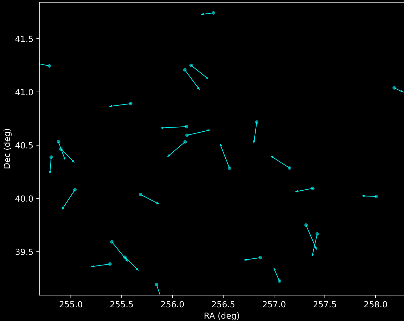
APOGEE DR17 Noise Stream Proper Motion Vectors (n=27)
